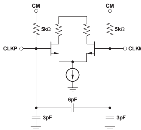
Figure 10. Clock Inputs
