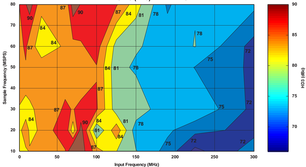
THIRD HARMONIC (HD3) WITH DLL OFF
