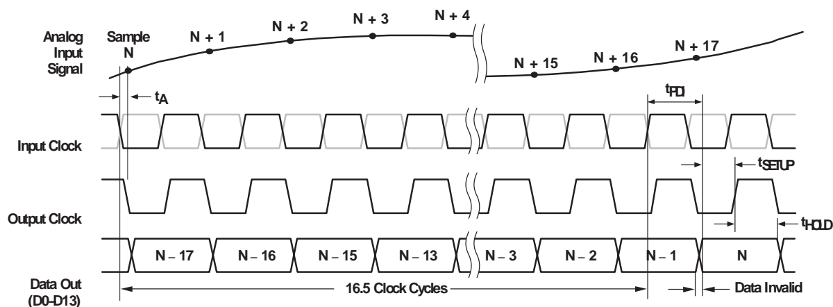
Figure 2. Timing Diagram
