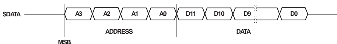
Figure 3. DATA Communication Is 2 Byte, MSB First
