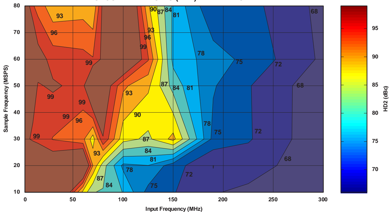
SECOND HARMONIC (HD2) WITH DLL OFF
