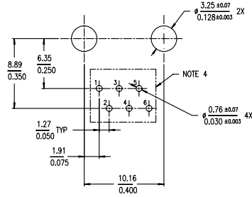
BOARD LAYOUT VIEWED FROM TOP
