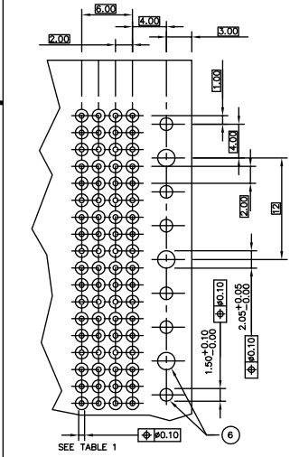
RECOMMENDED PC BOARD LAYOUT, COMPONENT SIDE.
