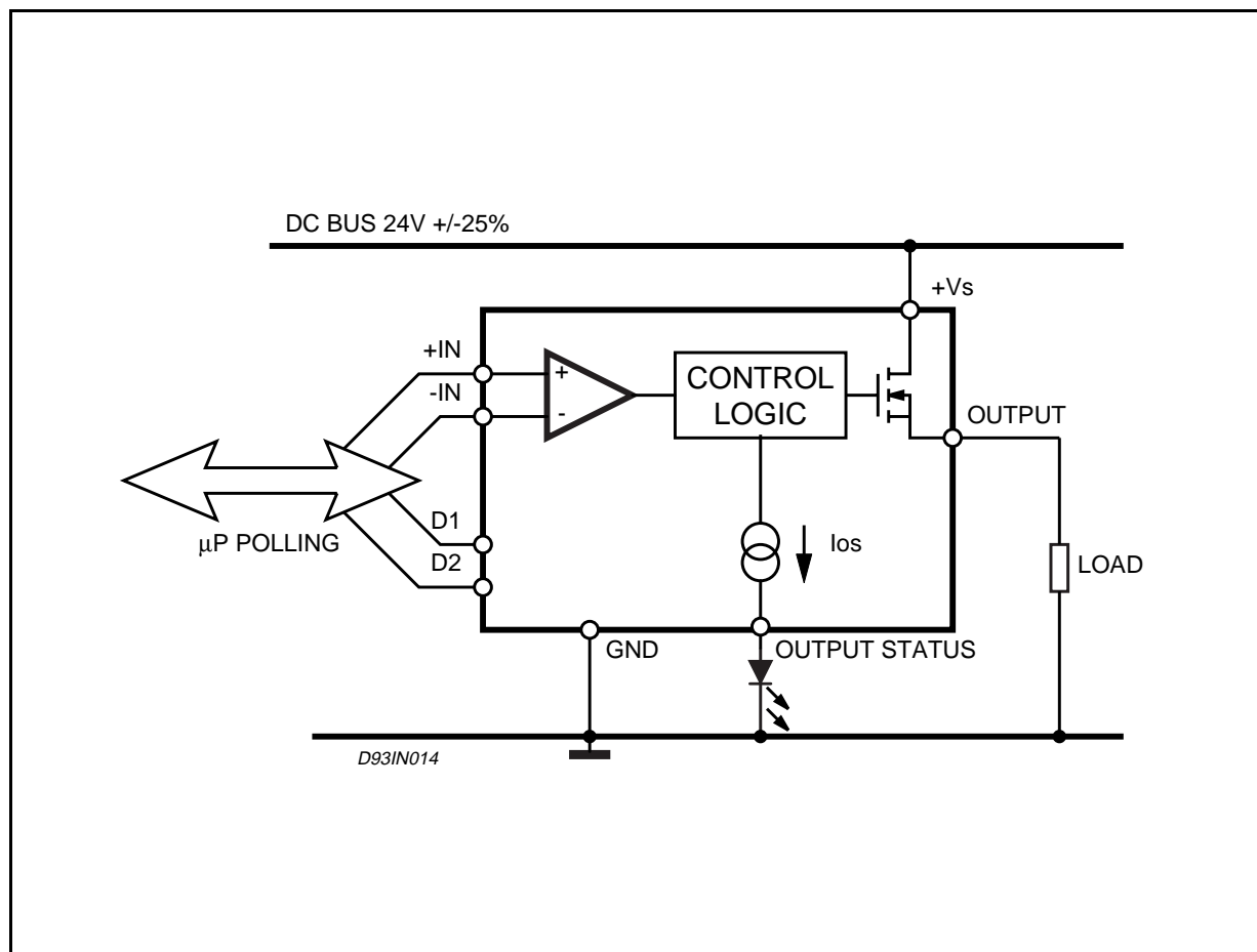
Figure 5: Application Circuit.
