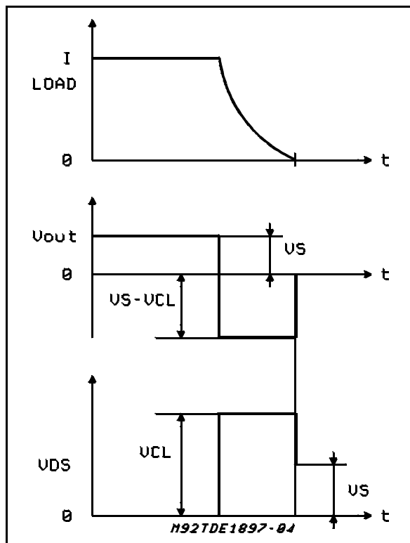
Figure 3: Demagnetization Cycle Waveforms
