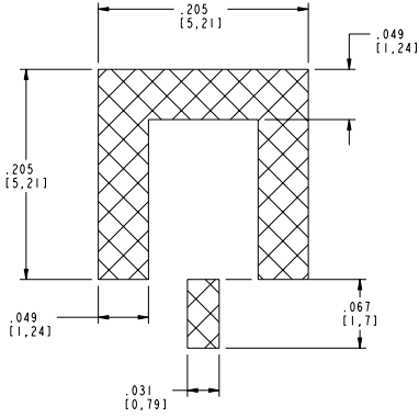
RECOMMENDED PCB FOOTPRINT SCALE 10.000
