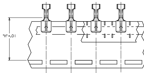
Ⓐ TAPE-MOUNTED PARTS
