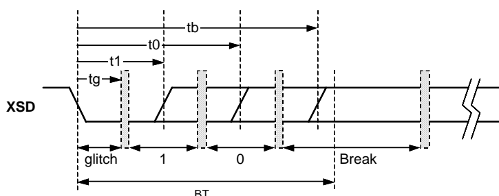
FIGURE 8. THE BUS SIGNAL TIMING DIAGRAM
