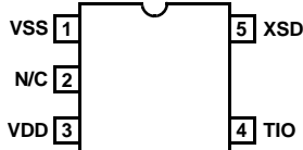
ISL6296 (5 LD SOT-23) TOP VIEW
