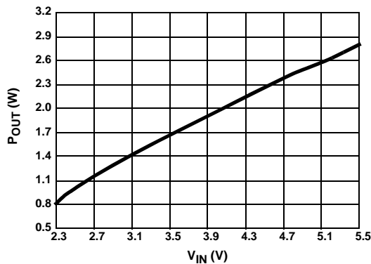
FIGURE 15. RECOMMENDED MAXIMUM OUTPUT POWER vs INPUT VOLTAGE
