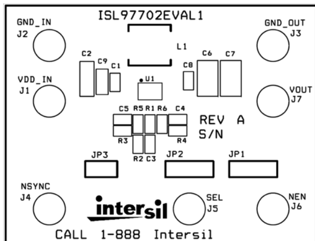
FIGURE 21. OVERVIEW of DEMO BOARD
