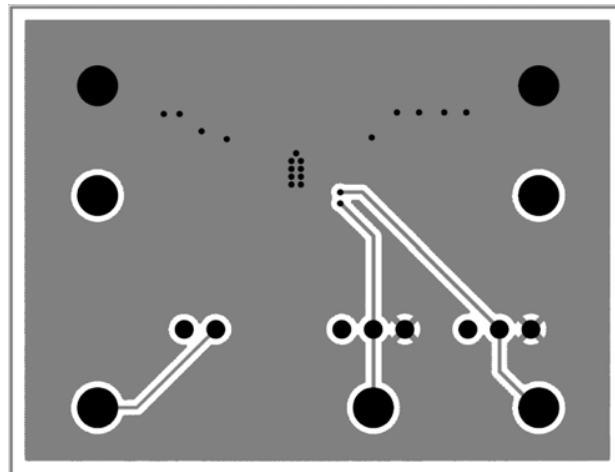
FIGURE 22. BOTTOM LAYER of the DEMO BOARD
