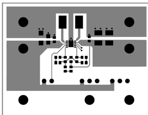
FIGURE 23. TOP LAYER of the DEMO BOARD
