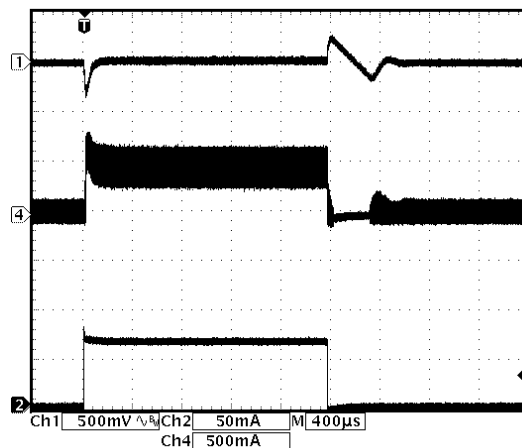
(CH1 = V_{OUT} ; CH4 = I_L ; CH2 = I_{OUT} )
