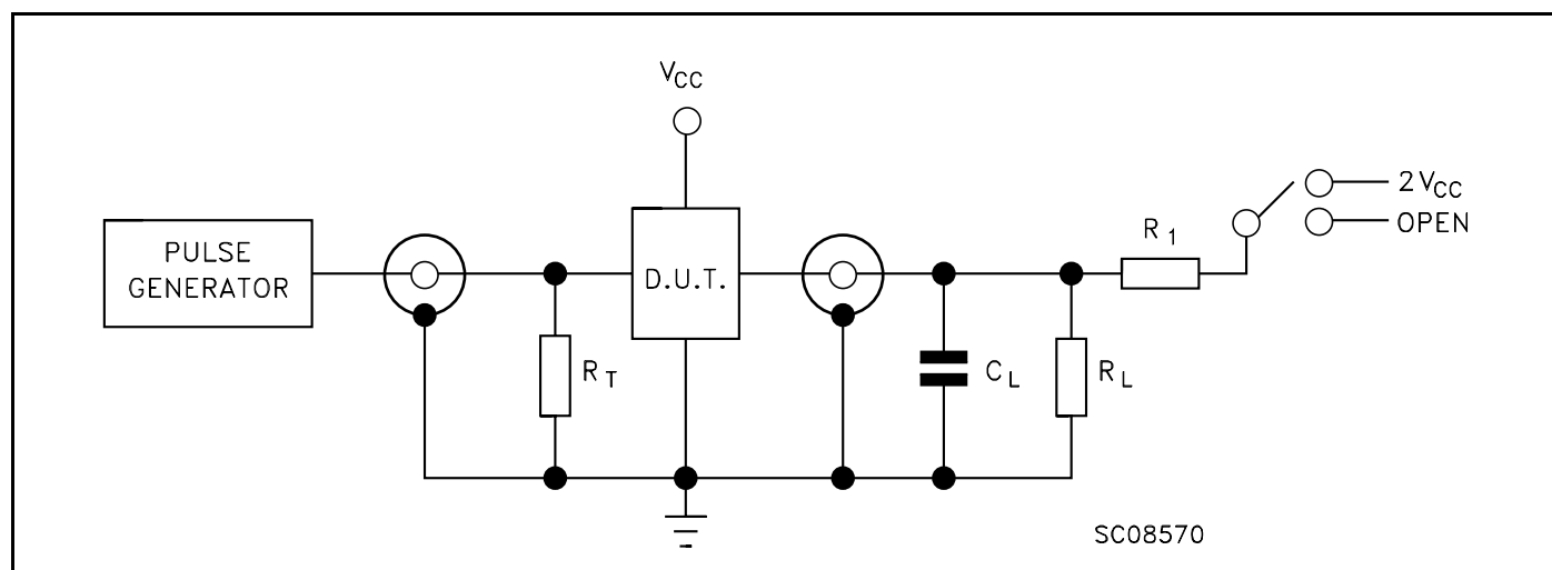
Figure 4: Test Circuit
