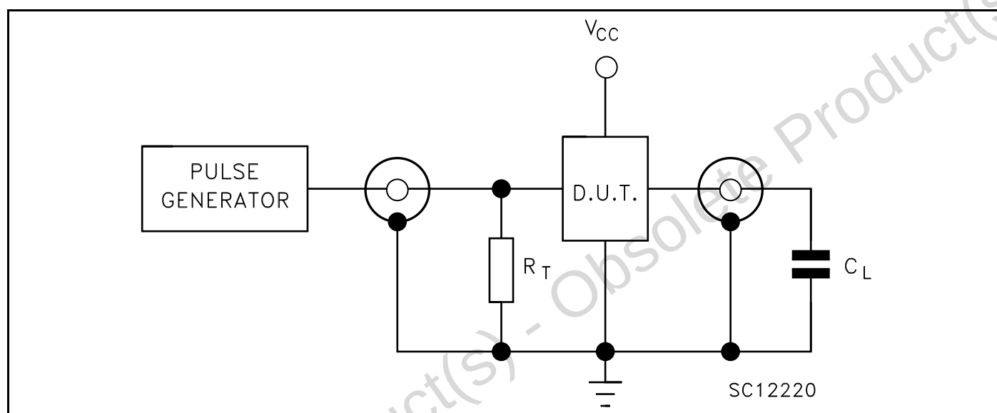
Figure 5: Test Circuit
