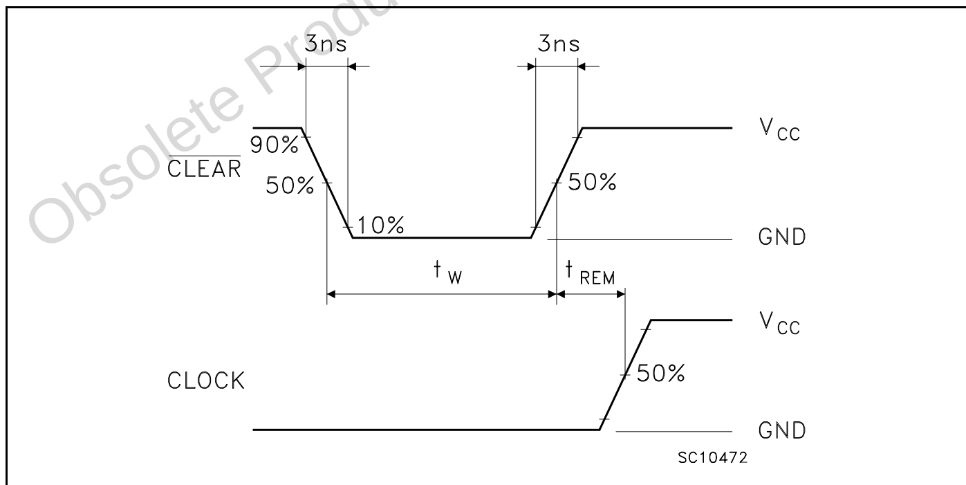
Figure 8: Waveform - Recovery Time ( f=1\text{MHz} ; 50% duty cycle)
