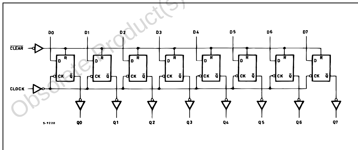
Figure 3: Logic Diagram
