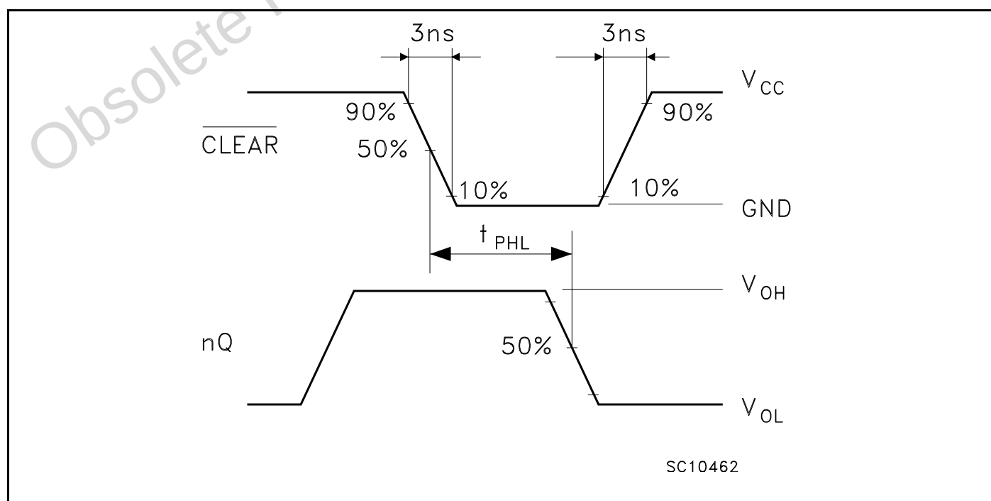
Figure 6: Waveform - Propagation Delays (f=1MHz; 50% duty cycle)
