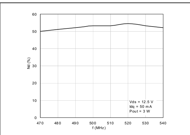
Figure 13. Efficiency vs frequency
