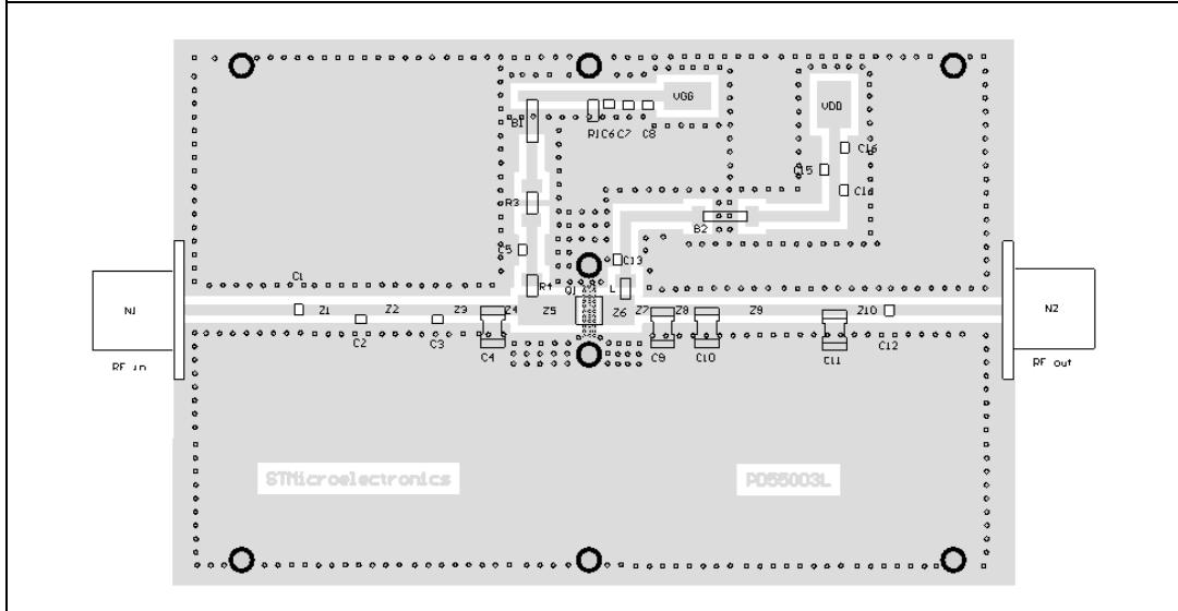
Figure 16. Test circuit
