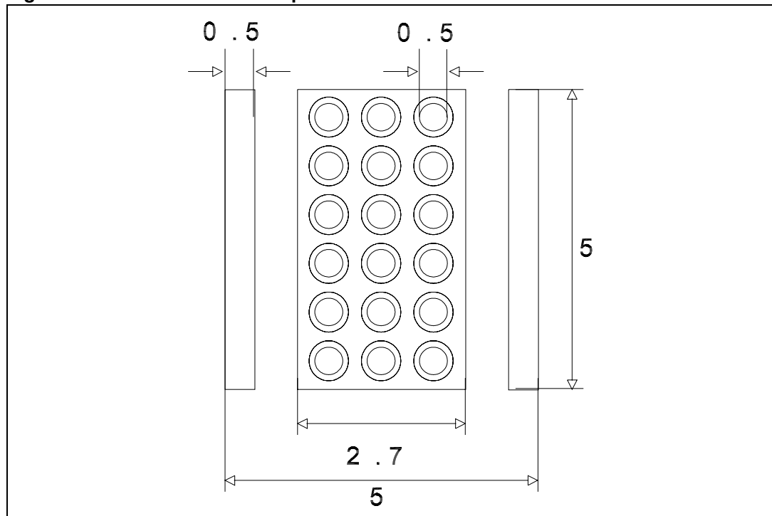
Figure 20. Recommended footprint
