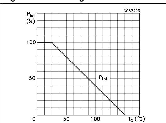
Figure 3. Derating curve
