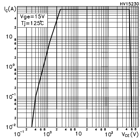
Figure 14. Turn-Off SOA
