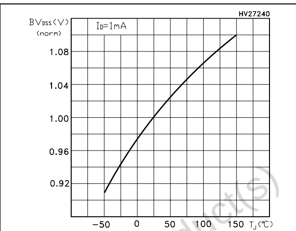
Figure 14. Normalized B_{V_{DS}} vs temperature
