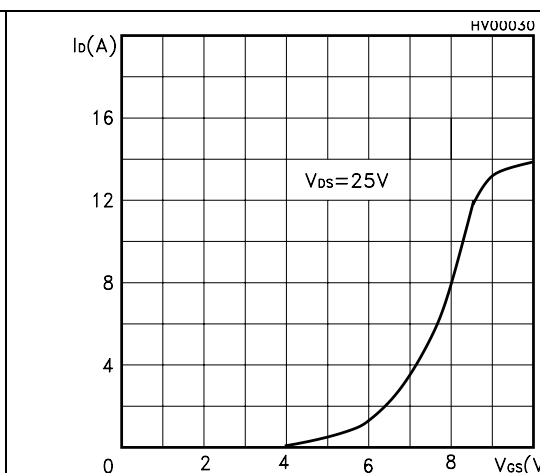
Figure 6. Transfer characteristics
