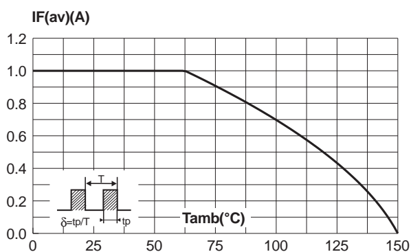
Fig. 2: Average forward current versus ambient temperature (δ=1).
