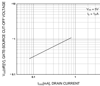
Figure 5. V_{GS(off)} - I_{DSS}
