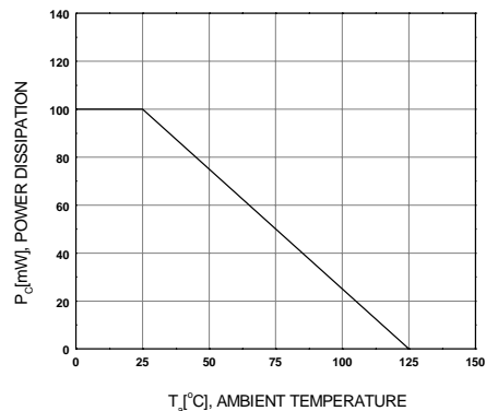
Figure 8. P_D - T_A
