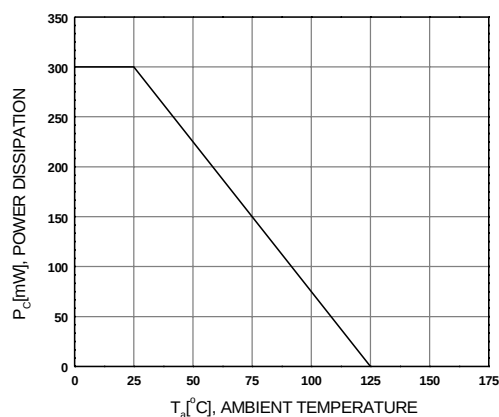
Figure 4. Power Derating
