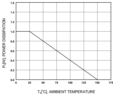
Figure 5. Power Derating
