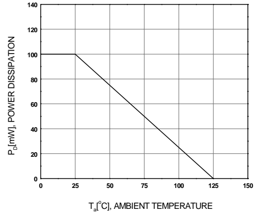
Figure 8. P_D - T_A
