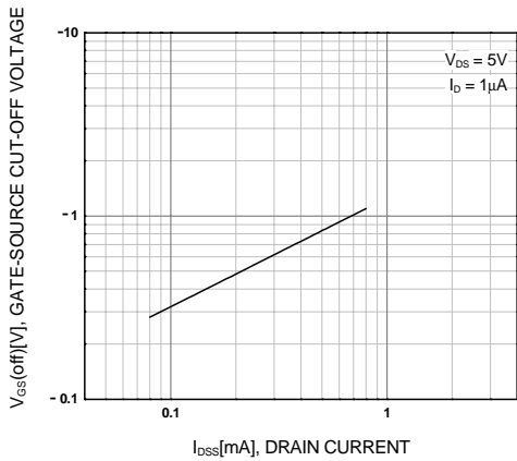
Figure 5. V_{GS(off)} - I_{DSS}
