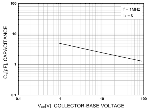
Figure 6. Reverse Capacitance
