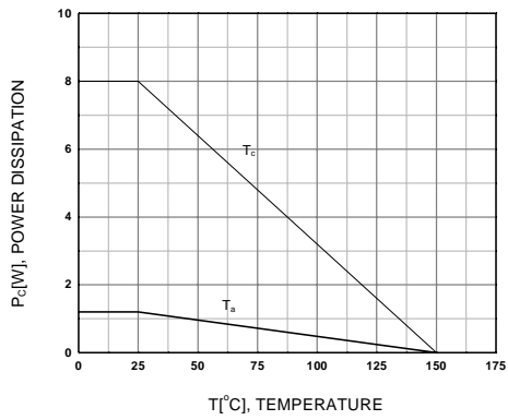
Figure 9. Power Derating
