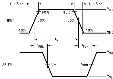
FIGURE 2. AC Waveforms
