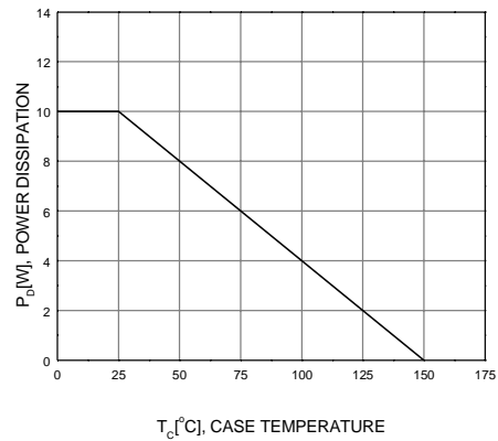
Figure 6. Power Derating
