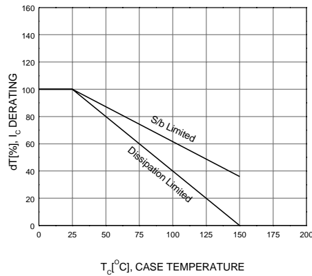
Figure 5. Derating Curve of Safe Operating Area
