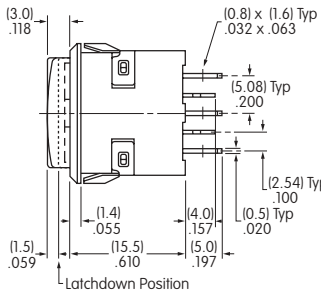
Single Color LED Side View
