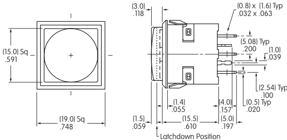
Bicolor LED Side View
