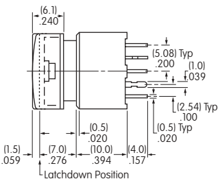
Bicolor LED Side View
