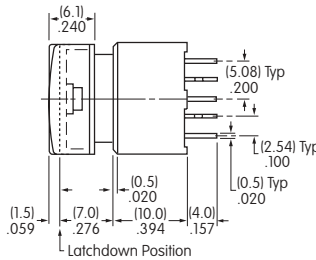
Single Color LED Side View
