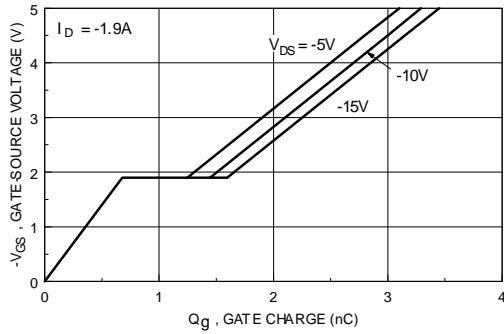
Figure 7. Gate-Charge Characteristics.
