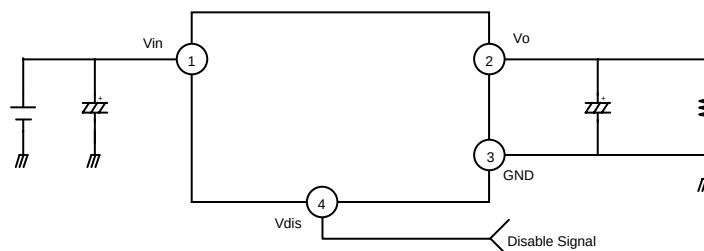
Figure 1. Application Circuit
