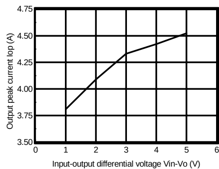
Figure 8. Output Peak Current vs. Input-Output Differential Voltage
