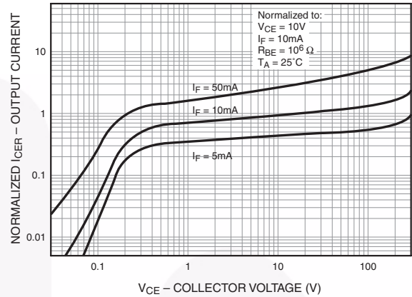
Fig. 2 Normalized Output Characteristics
