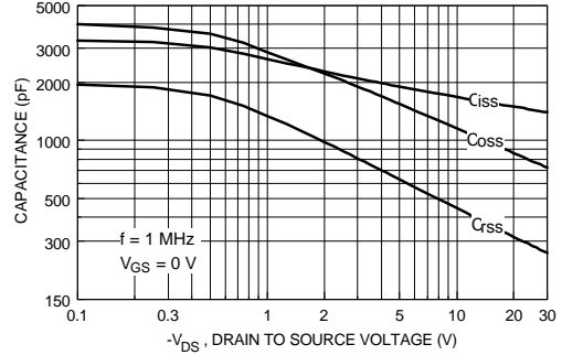
Figure 8. Capacitance Characteristics.
