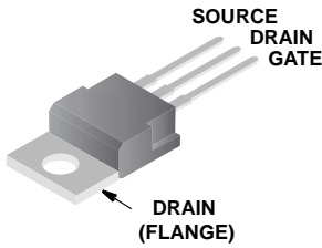
HUFA76633P3
