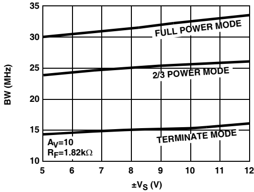
FIGURE 31. DIFFERENTIAL BANDWIDTH vs SUPPLY VOLTAGE
