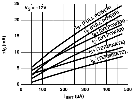
FIGURE 35. I_S vs I_{SET}
