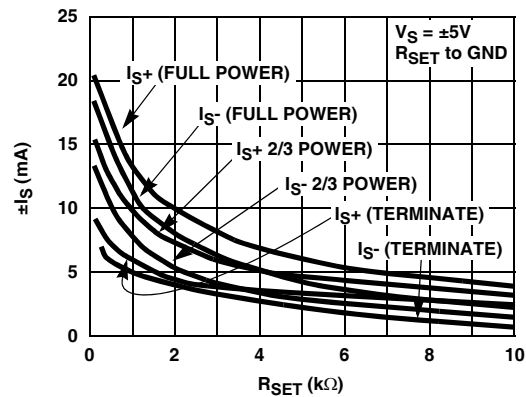
FIGURE 34. IS vs RSET
