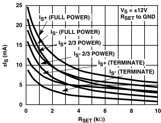
FIGURE 33. IS vs RSET
