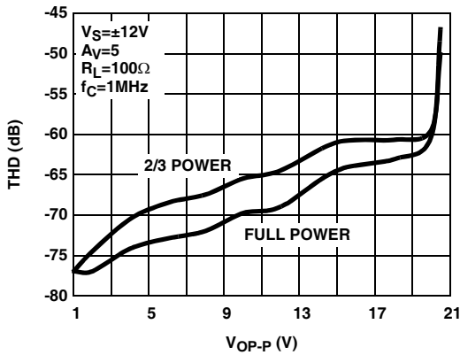
FIGURE 23. DIFFERENTIAL TOTAL HARMONIC DISTORTION vs OUTPUT AMPLITUDE
