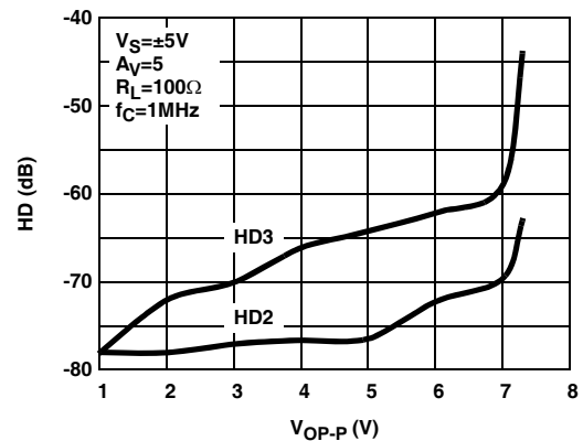
FIGURE 22. DIFFERENTIAL HARMONIC DISTORTION vs OUTPUT AMPLITUDE
