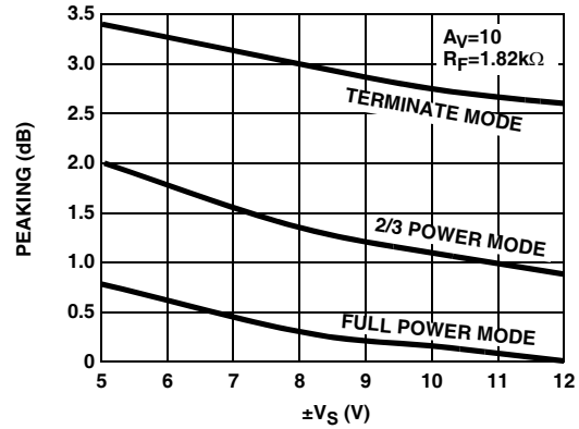
FIGURE 32. DIFFERENTIAL PEAKING vs SUPPLY VOLTAGE
