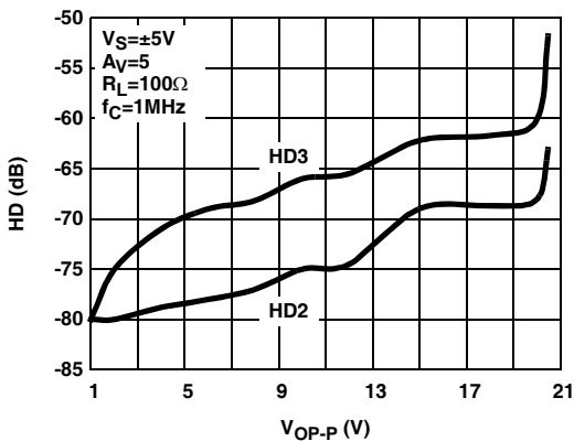
FIGURE 21. DIFFERENTIAL HARMONIC DISTORTION vs OUTPUT AMPLITUDE (2/3 POWER)
