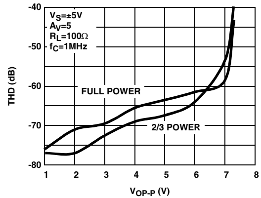
FIGURE 24. DIFFERENTIAL TOTAL HARMONIC DISTORTION vs OUTPUT AMPLITUDE
