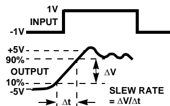
SLEW RATE
