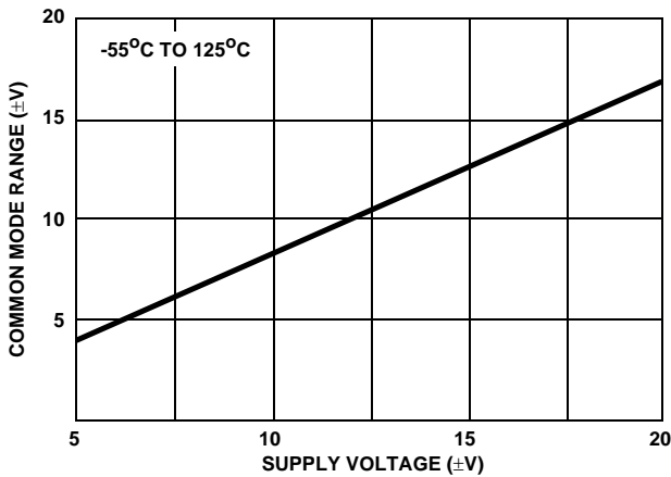
FIGURE 10. COMMON MODE VOLTAGE RANGE vs SUPPLY VOLTAGE
