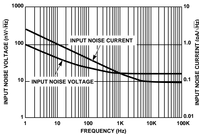
FIGURE 12. NOISE DENSITY vs FREQUENCY
