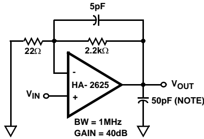
FIGURE 3. VIDEO AMPLIFIER
