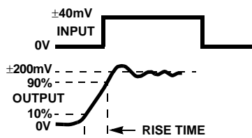
TRANSIENT RESPONSE
