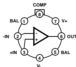
HA-2620 (METAL CAN) TOP VIEW
