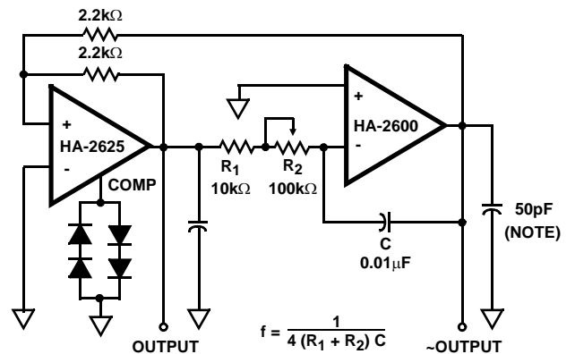
FIGURE 2. FUNCTION GENERATOR
