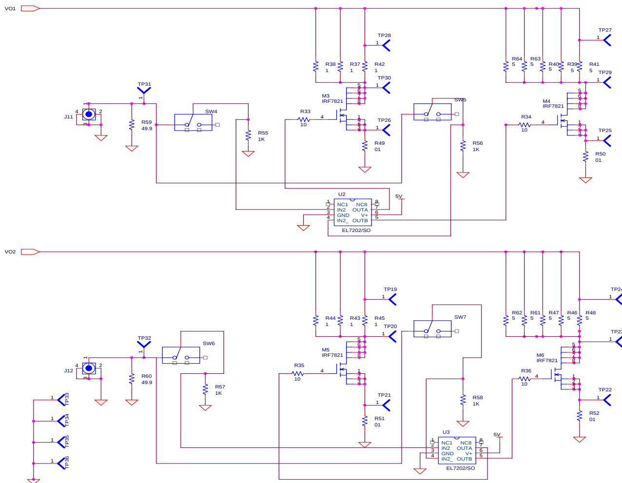
FIGURE 39. EVAL BOARD SCHEMATIC (CONTINUED)
