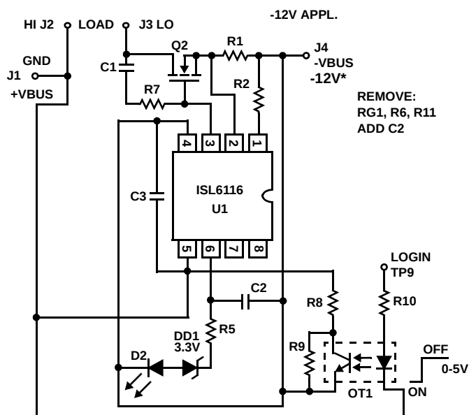
FIGURE 6. ISL6116EVAL1 NEGATIVE VOLTAGE LOW SIDE CONTROLLER
