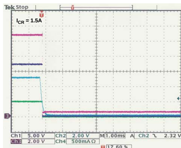
FIGURE 20. TURN OFF VIA PWRON
