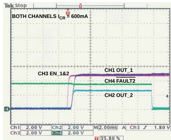
FIGURE 66. TURN ON INTO SHORT
