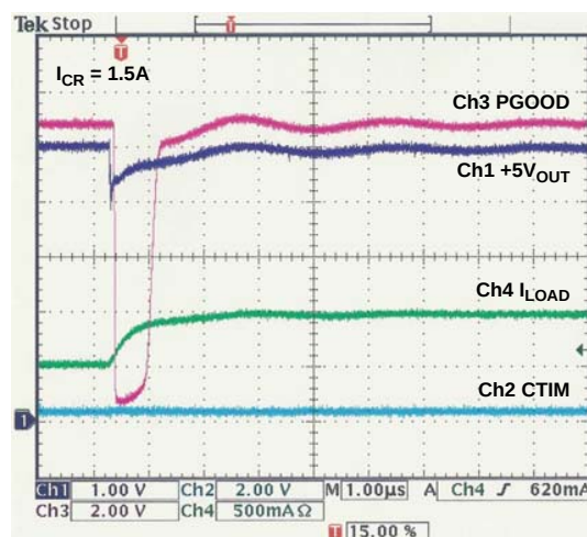
FIGURE 5B. RESPONSE TO FALSE FAULT EVENT
