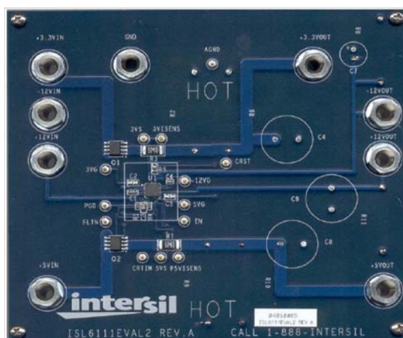
FIGURE 53. EVAL BOARD PICTURE
