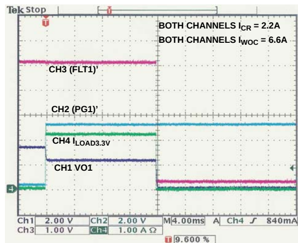
FIGURE 44. RESPONSE TO OC IN LATCH MODE ((PG)')
