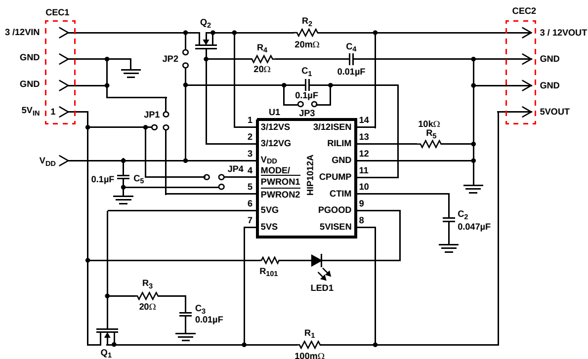
FIGURE 36. SCHEMATIC FOR +5V AND +12V OPERATION
