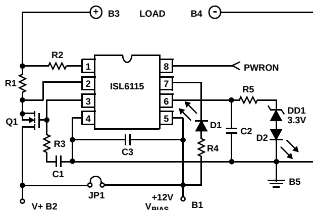
FIGURE 17. ISL6115 EVAL BOARD SCHEMATIC
