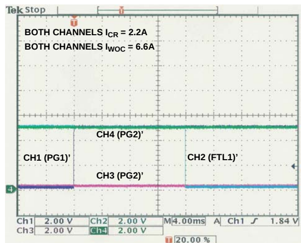
FIGURE 46. OC CHANNEL COMPARISON ((FLT)') AND ((PG)')
