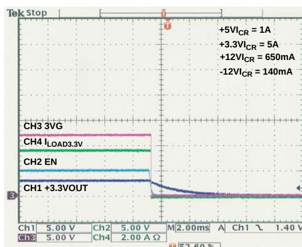
FIGURE 57. TURN OFF SHOWING +3.3V DETAILS
