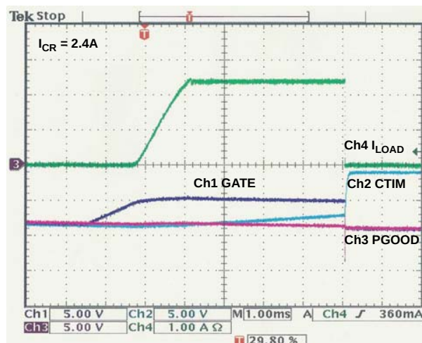
FIGURE 9. TURN ON INTO OVERCURRENT
