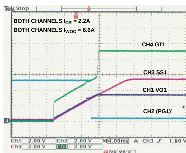
FIGURE 42. TURN ON SHOWING CHANNEL 1 DETAILS
