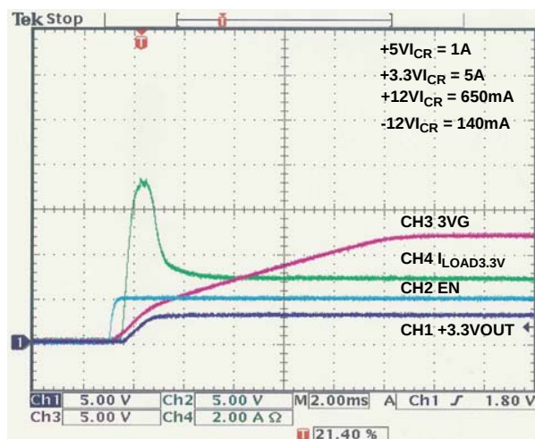
FIGURE 55. TURN ON SHOWING +3.3V DETAILS
