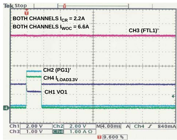
FIGURE 48. OC WITH RECOVERY BEFORE TIMEOUT ((PG)')
