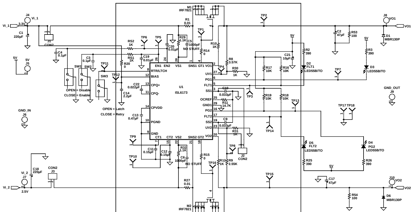
FIGURE 38. EVAL BOARD SCHEMATIC
