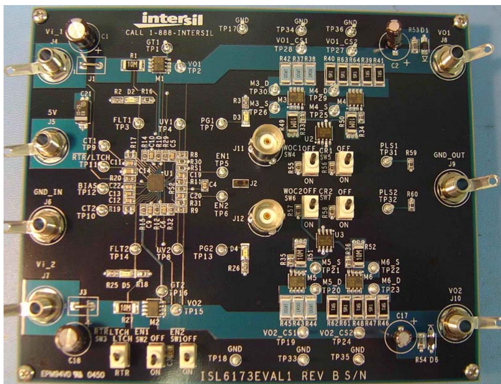
FIGURE 40. ISL6173 EVAL BOARD PICTURE
