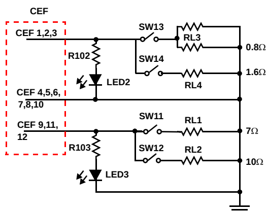
FIGURE 25. LOAD CIRCUIT SCHEMATIC
