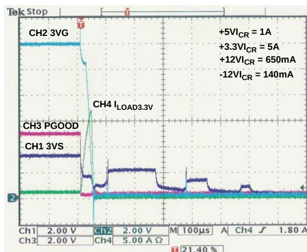
FIGURE 59. RESPONSE TO OC ON +3.3V CHANNEL
