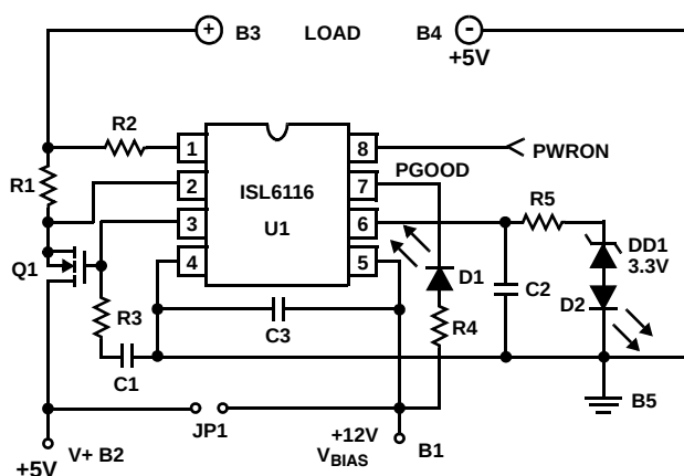
FIGURE 1. EVAL BOARD SCHEMATIC
