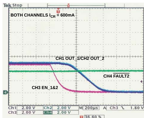
FIGURE 64. TURN OFF VIA EN
