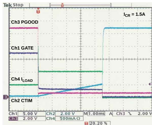
FIGURE 22. RESPONSE TO OC DURING OPERATION
