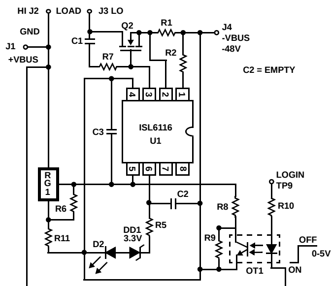
FIGURE 11. ISL6116 EVAL BOARD SCHEMATIC
