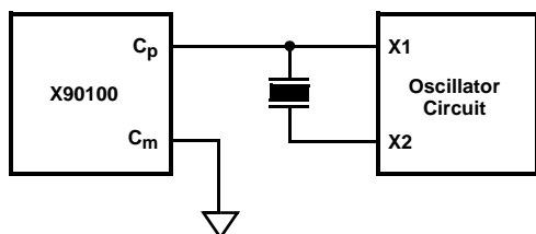
Example of a single-ended circuit
