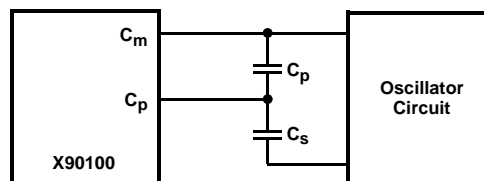
Example of a differential mode circuit
