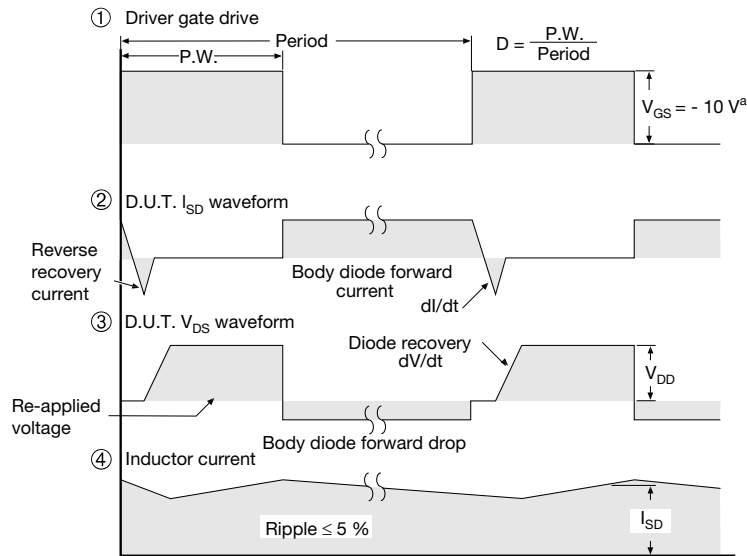
Fig. 14 - For P-Channel
