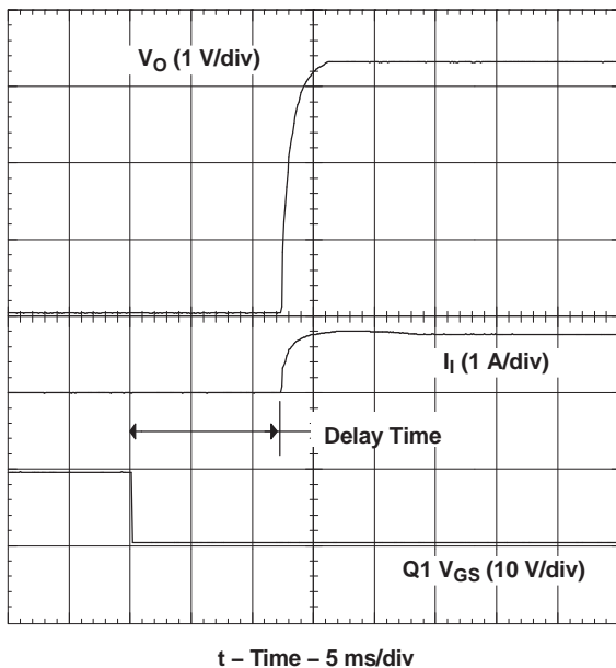
Figure 14. Power Up
