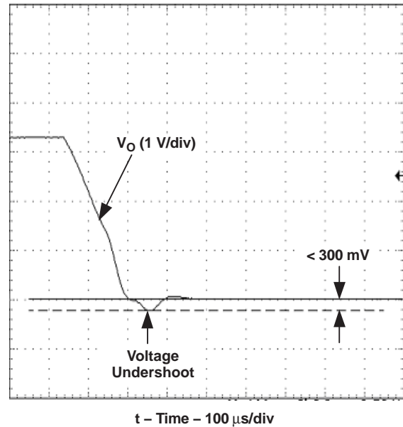
Figure 15. Power Down
