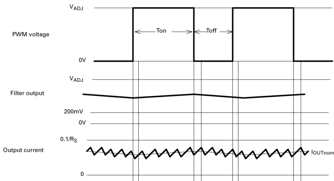
Figure 3. High Frequency PWM operating waveforms
