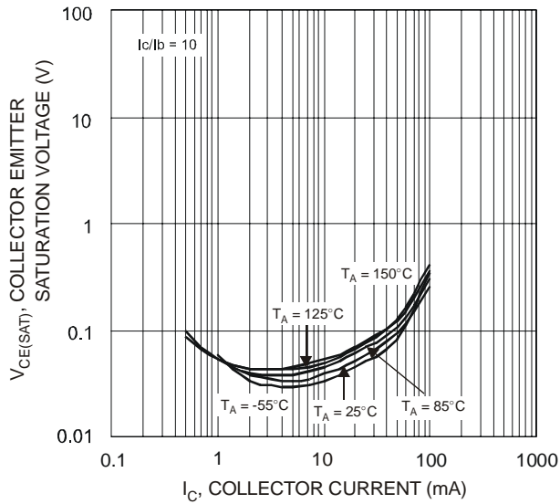
Fig. 9 I_C vs. V_{CE(SAT)}
