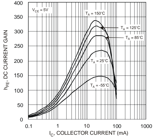
Fig. 3 DC Current Gain vs. I_C
