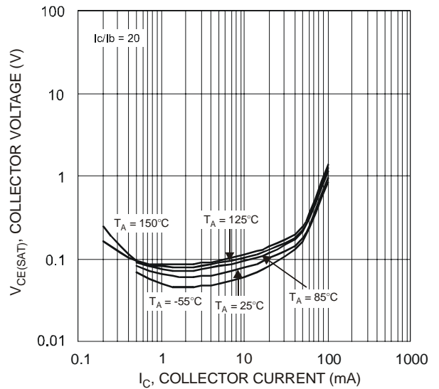
Fig. 5 I_C vs. V_{CE(SAT)}
