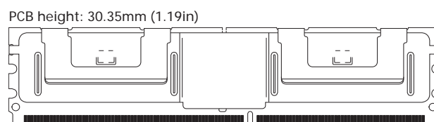
Figure 1: 240-Pin FBDIMM (MO-256 R/C C)
