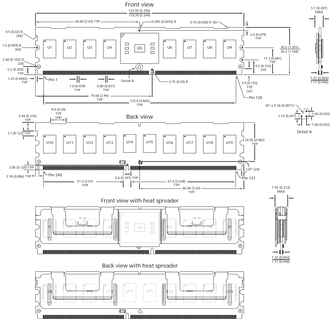
Figure 4: 240-Pin DDR2 FBDIMM
