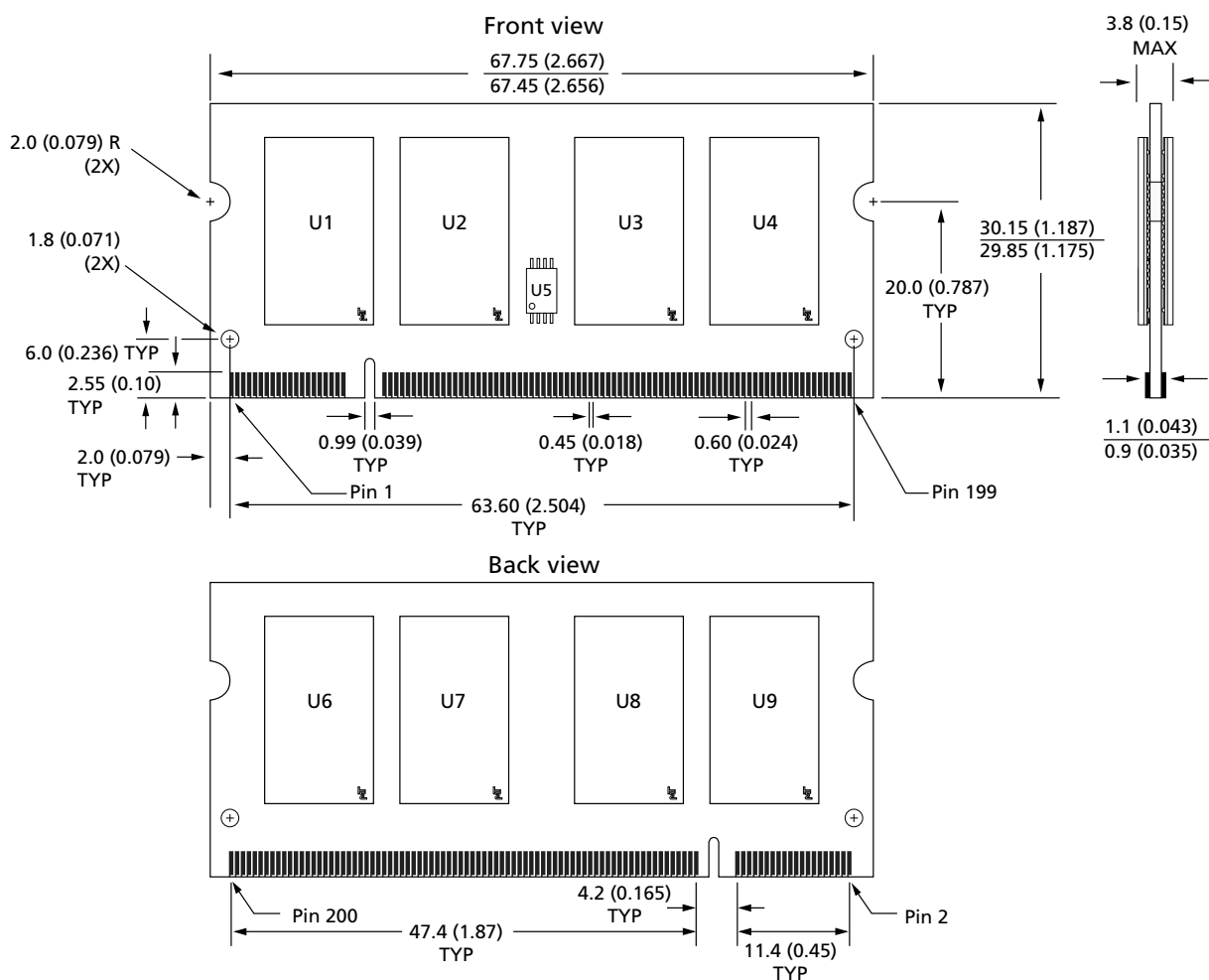
Figure 3: 200-Pin DDR2 SODIMM
