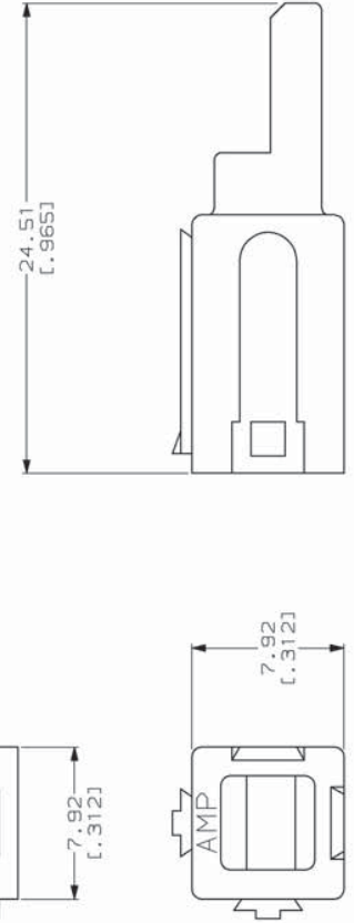
DETAIL B
