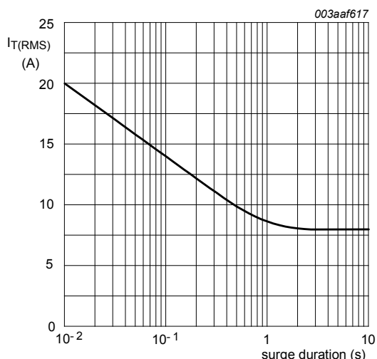
Fig. 2. RMS on-state current as a function of surge duration; maximum values f = 50\text{ Hz} ; T_{mb} = 102\text{ }^{\circ}\text{C}
