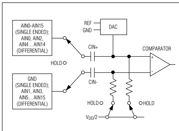
Figure 3. Equivalent Input Circuit
