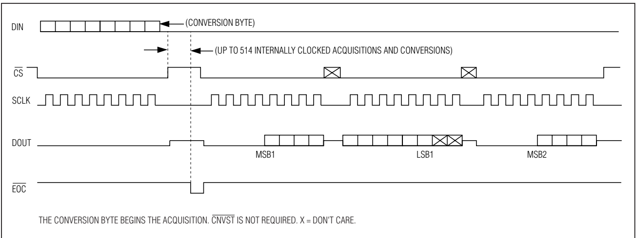
Figure 6. Clock Mode 10
