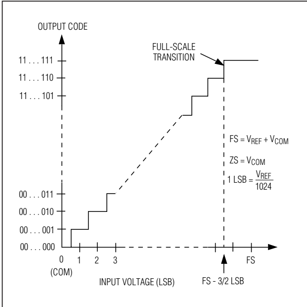
Figure 8. Unipolar Transfer Function, Full Scale (FS) = VREF
