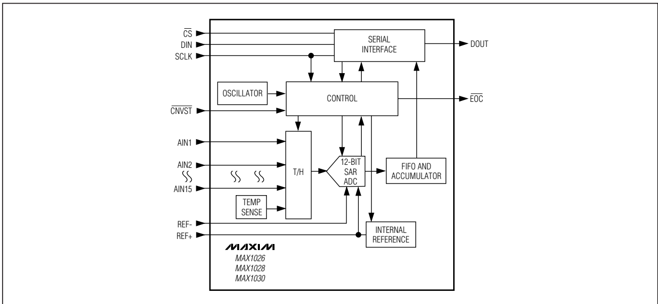
Figure 2. Functional Diagram
