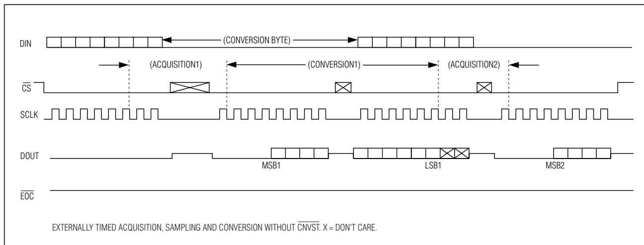
Figure 7. Clock Mode 11
