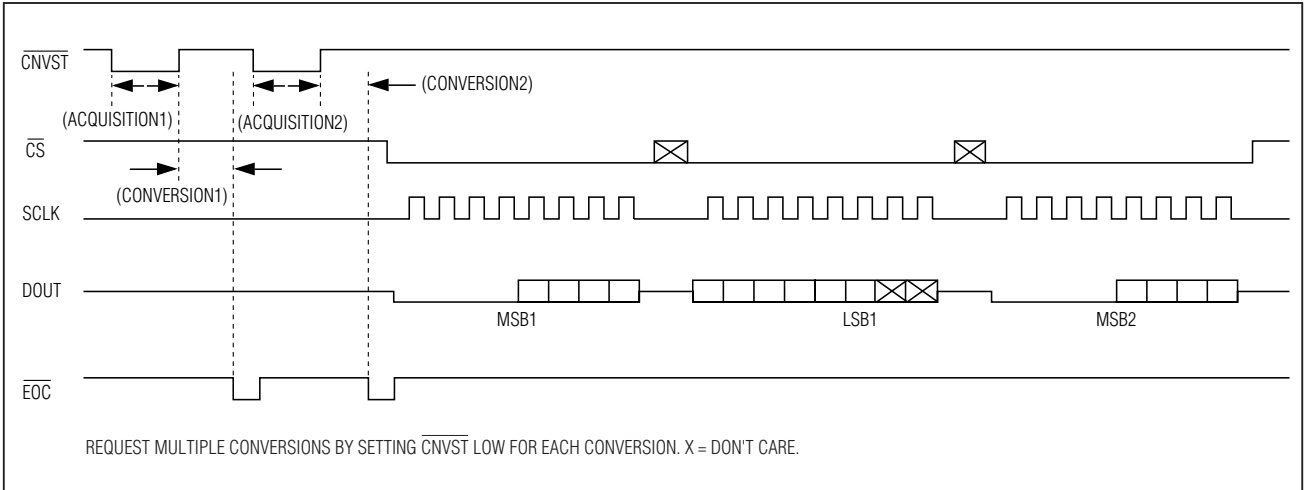
Figure 5. Clock Mode 01
