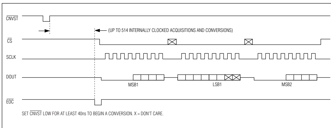
Figure 4. Clock Mode 00
