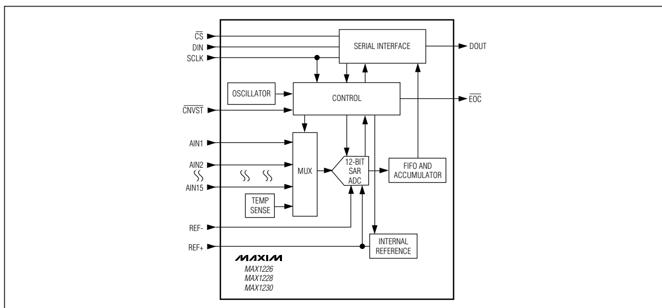
Figure 2. Functional Diagram
