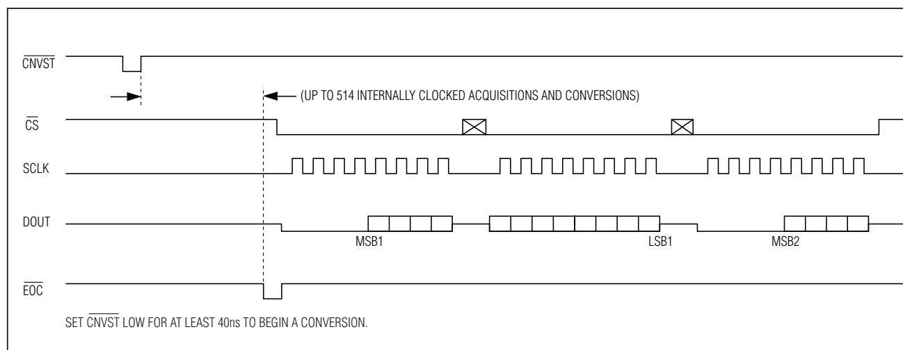
Figure 4. Clock Mode 00
