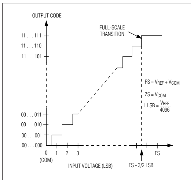
Figure 8. Unipolar Transfer Function, Full Scale (FS) = V_{REF}
