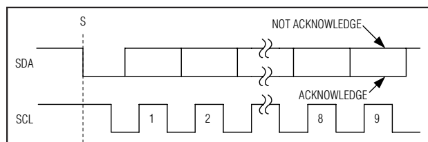
Figure 6. Acknowledge Bits
