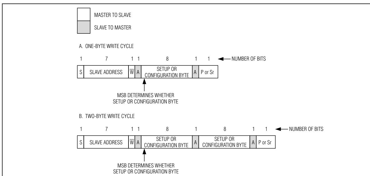
Figure 9. Write Cycle
