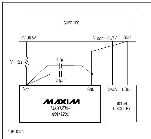
Figure 14. Power-Supply Grounding Connection
