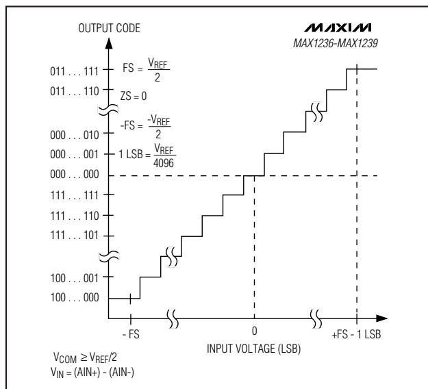
Figure 13. Bipolar Transfer Function
