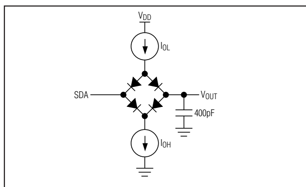
Figure 3. Load Circuit
