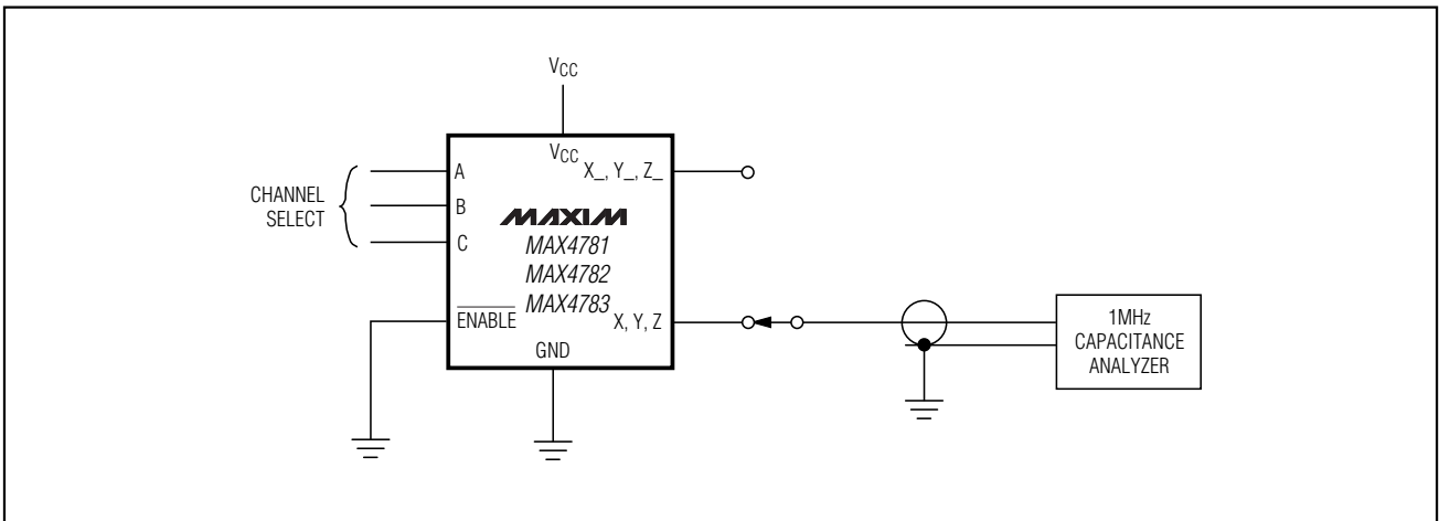
Figure 6. Capacitance
