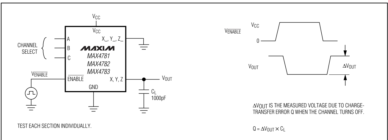
Figure 4. Charge Injection
