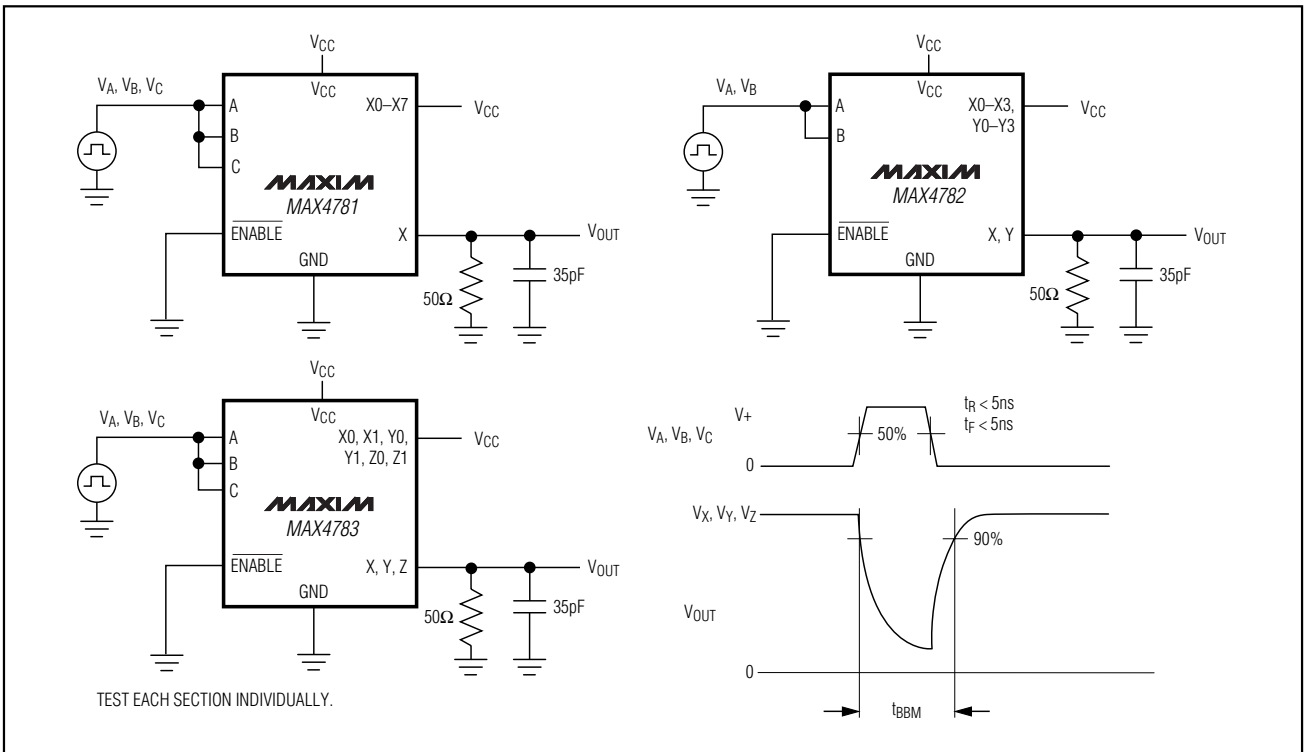
Figure 3. Break-Before-Make Interval
