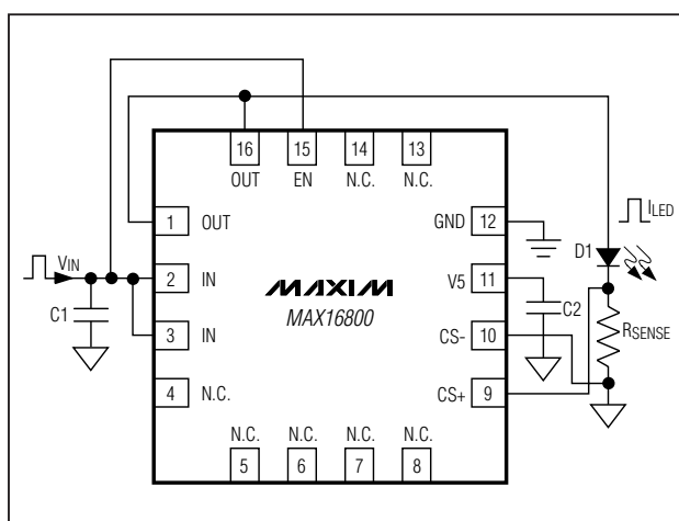
Figure 2. Pulse Application with EN Connected to V_{IN}
