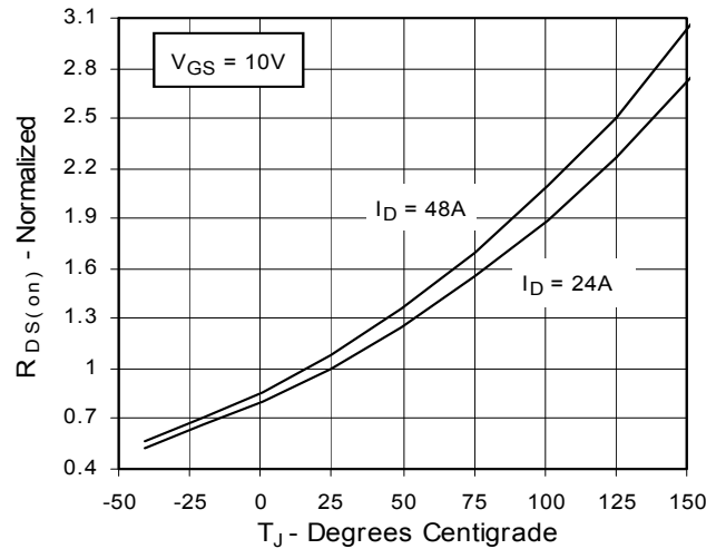
Fig. 4. R_{DS(on)} Normalized to I_D = 24\text{A} Value vs. Junction Temperature
