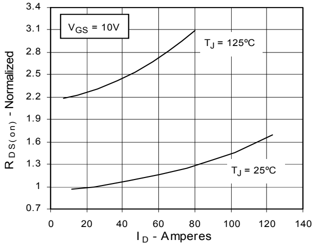
Fig. 5. R_{DS(on)} Normalized to I_D = 24\text{A} Value vs. Drain Current
