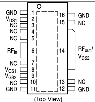
Figure 2. Pin Connections
