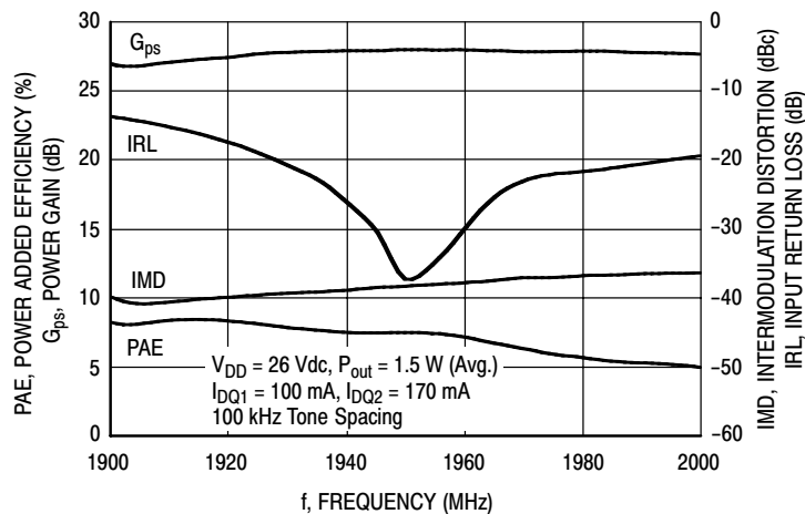
Figure 6. Two-Tone Wideband Performance @ P_{out} = 1.5 Watts Avg.
