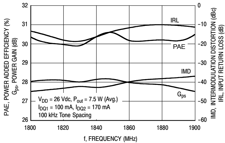
Figure 23. Two-Tone Wideband Performance @ P out = 7.5 Watts Avg.
