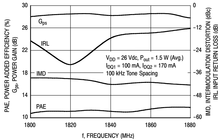
Figure 24. Two-Tone Wideband Performance @ P out = 1.5 Watts Avg.
