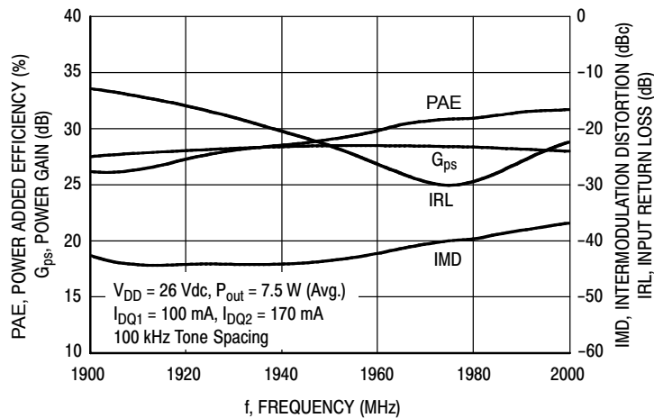
Figure 5. Two-Tone Wideband Performance @ P_{out} = 7.5 Watts Avg.
