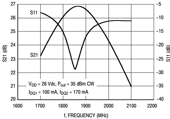
Figure 32. Broadband Frequency Response
