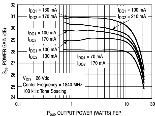
Figure 25. Two-Tone Power Gain versus Output Power
