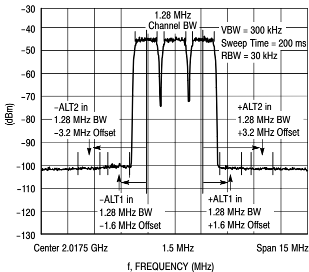
Figure 41. 3-Carrier TD-SCDMA Spectrum
