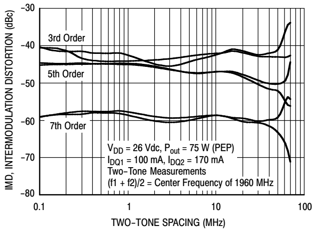
Figure 9. Intermodulation Distortion Products versus Tone Spacing
