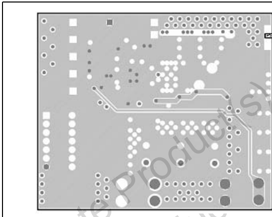
Figure 9. PCB layout - Signal-ground layer
