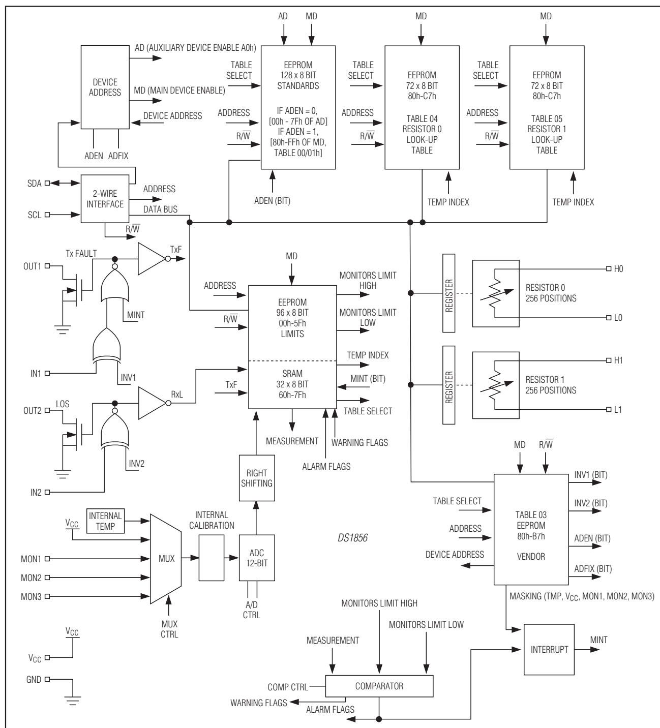
Figure 1. Block Diagram
