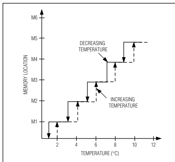
Figure 4. Look-Up Table Hysteresis
