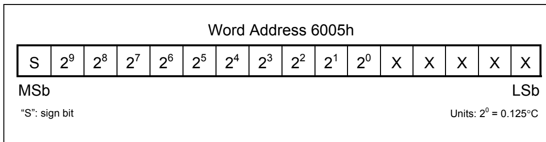
Figure 16. Temperature Register Format
