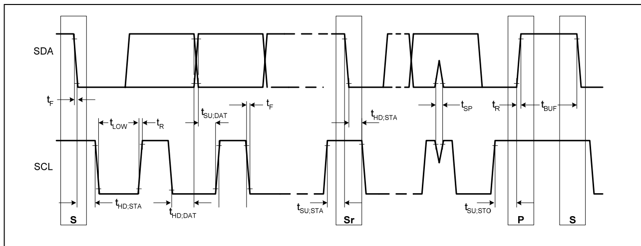
Figure 1. 2-Wire Bus Timing Diagram
