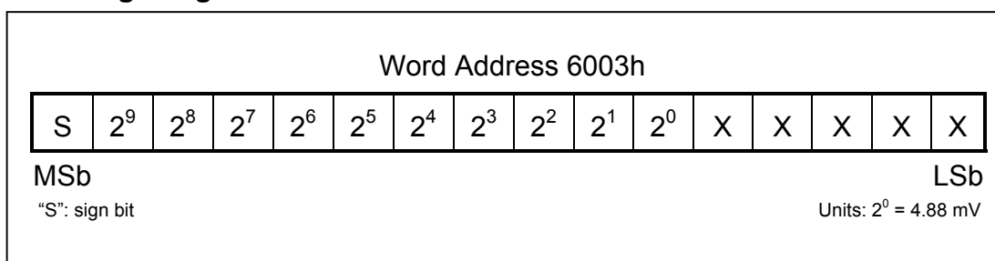
Figure 15. Voltage Register Format
