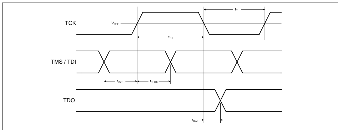
Figure 2. JTAG Timing Diagram
