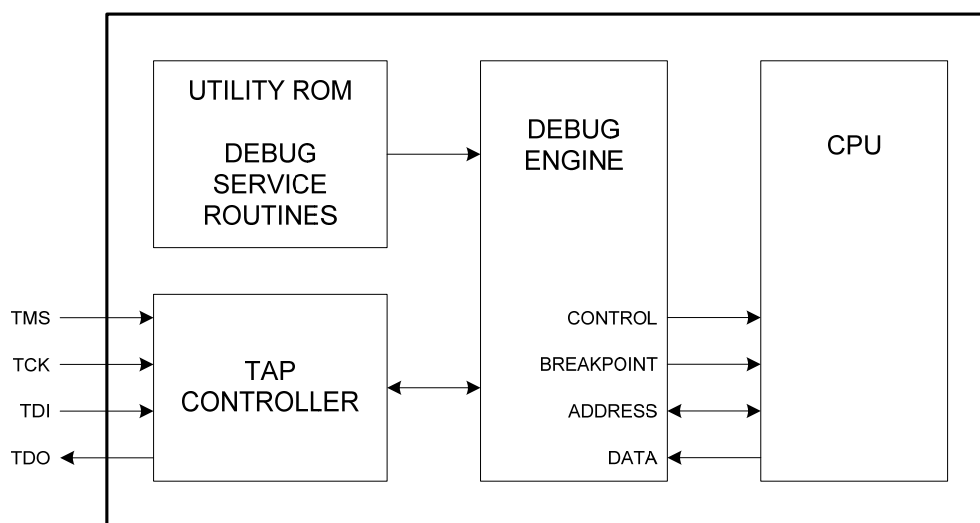
Figure 21. In-Circuit Debugger
